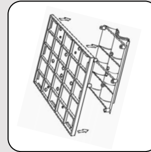
Fixing of basic frame to pipe-bracket
