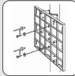
Top frame and bracket, fixed to sign-pipe with screws or pop-rivets
